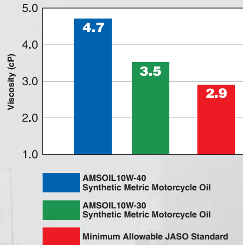
High-Temperature Viscosity Protection (ASTM D4683)
